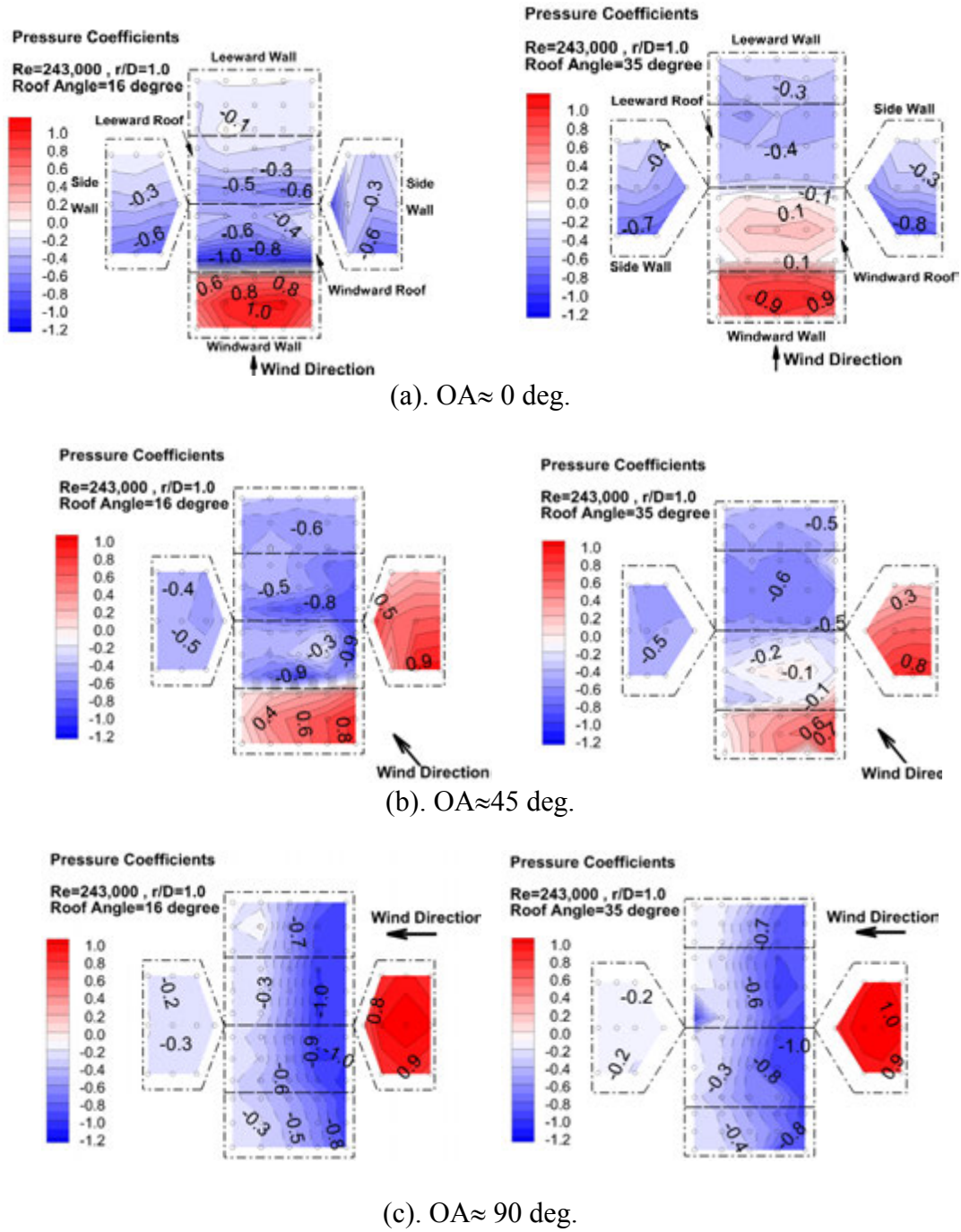
Figure 11. The pressure distributions around the building models at different orientation angles. (left: building model with 16 degree roof angle; right: building model with 35 degree roof angle)
