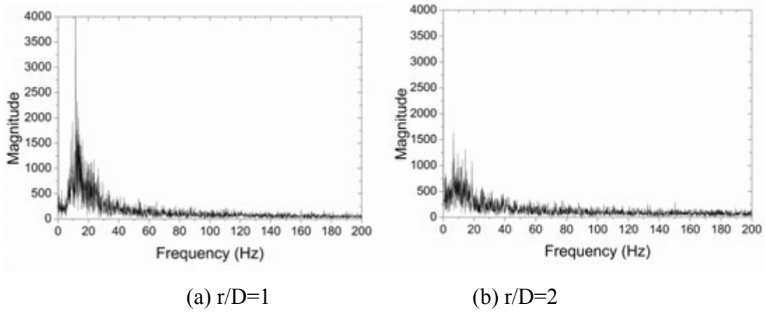
Figure 11. Frequency spectrum of the radial-velocity fluctuation at z/D=0.20 (Experiment, Cobra-probe)
