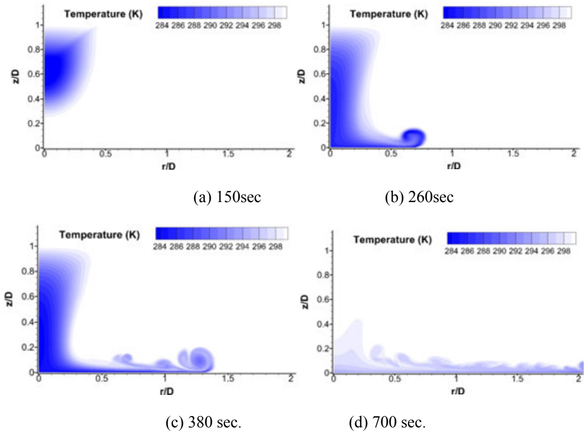
Figure 7. Evolution of the temperature field in cooling source model (Numerical Simulation)
