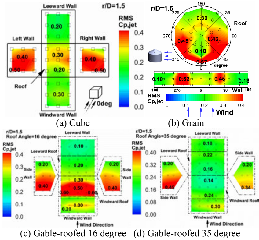
Figure 8. Comparison of RMS pressure coefficient at r/D \approx 1.5
